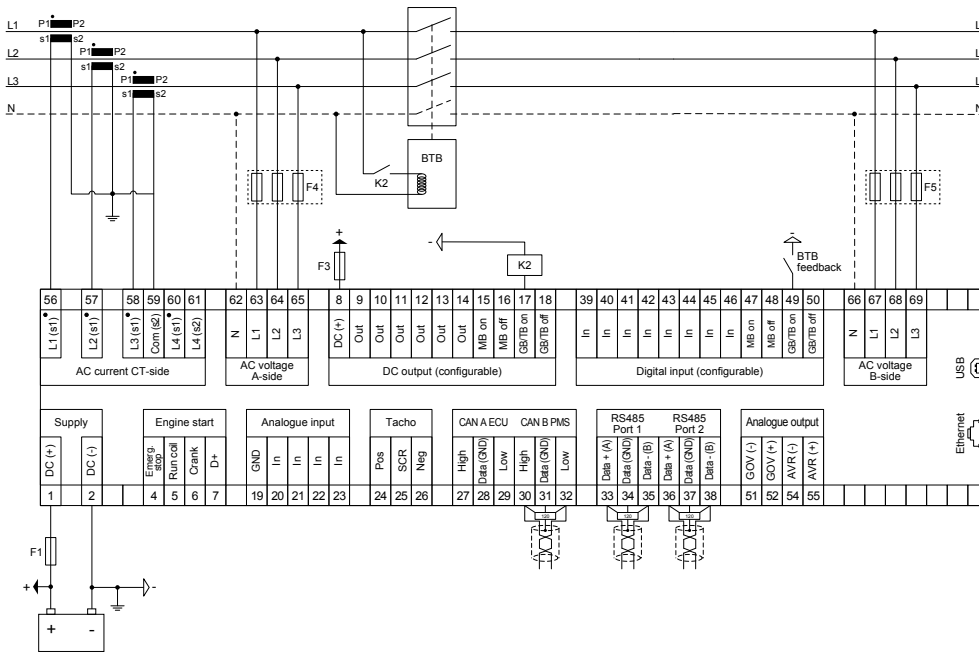
Figure 5.4 Typical wiring for hybrid
