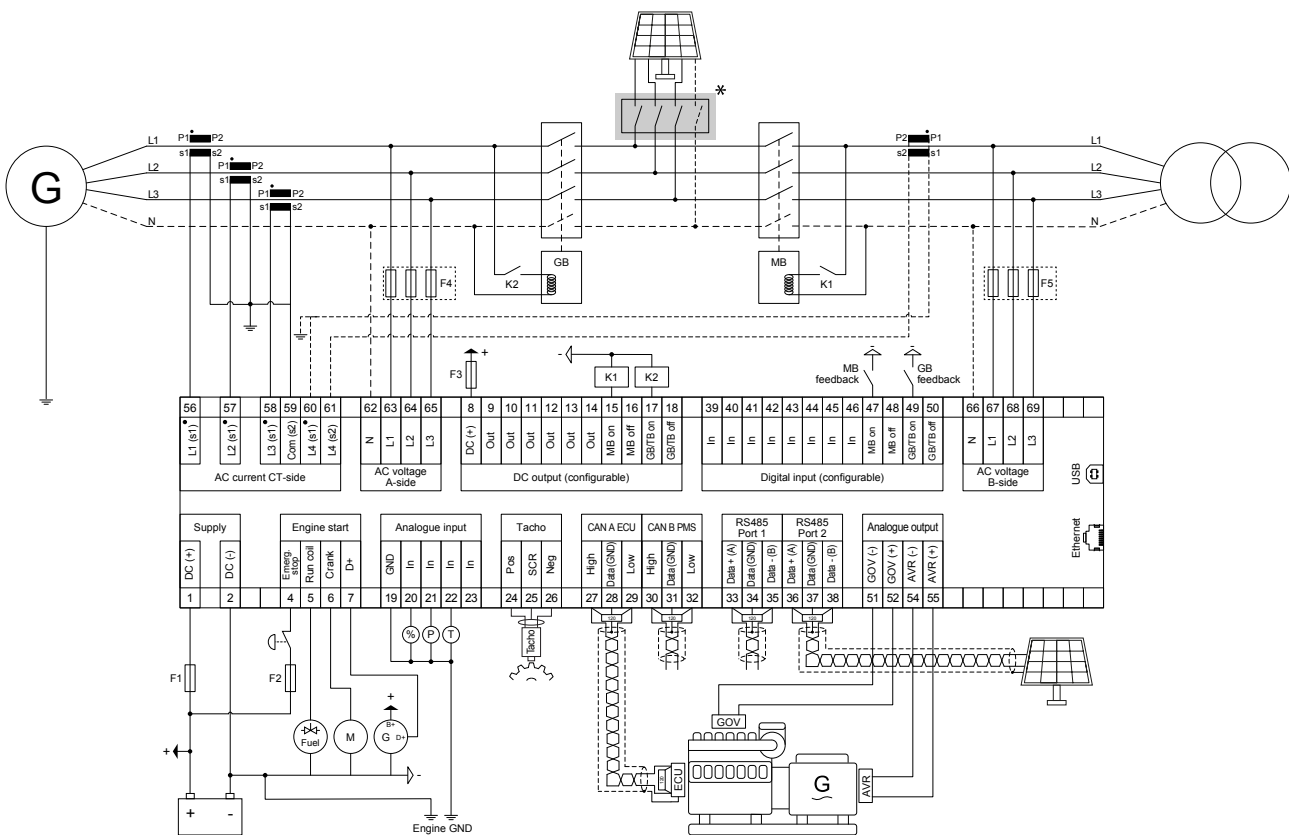
Figure 5.4 Typical wiring for hybrid
