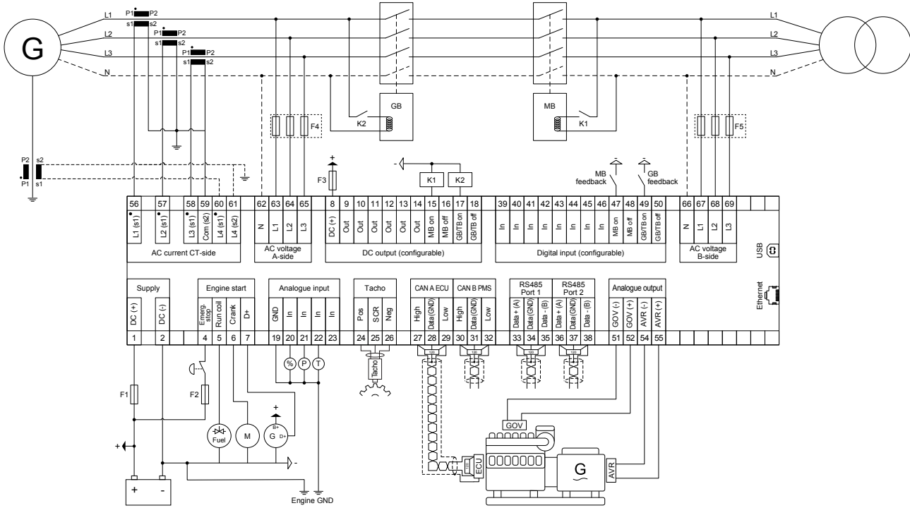
Figure 5.1 Typical wiring for genset
